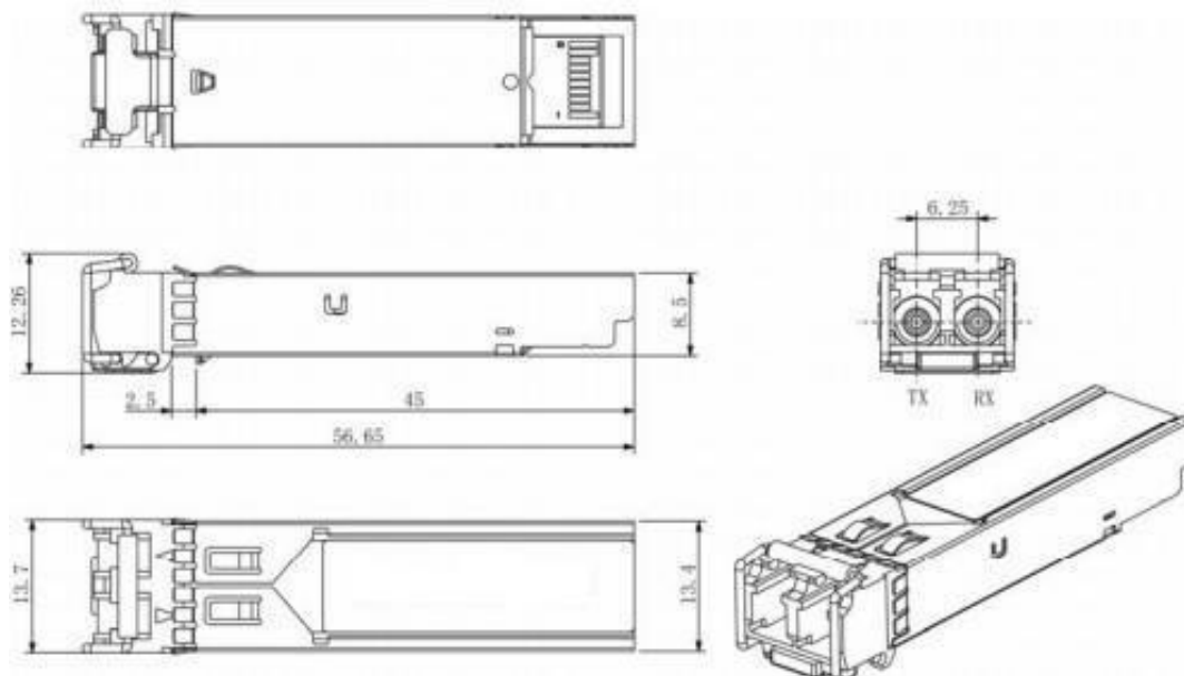
Mechanical Drawing
